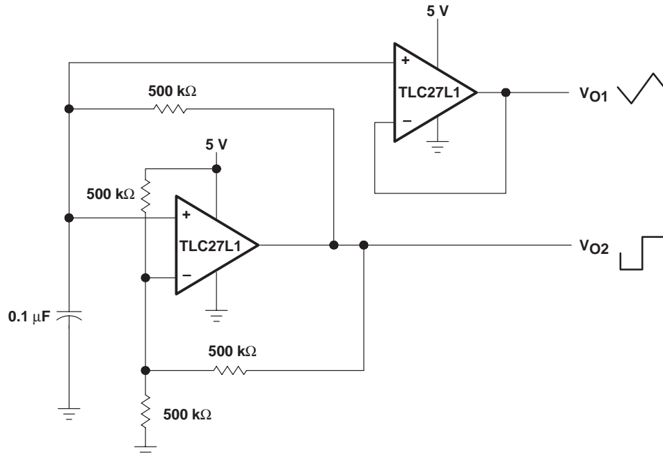
Figure 49. Multivibrator
