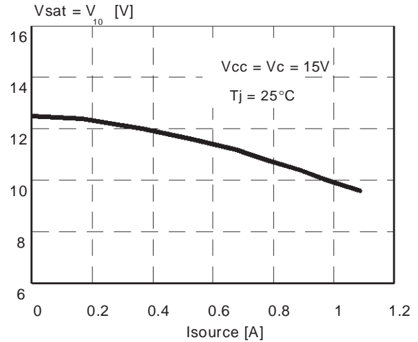
Figure 12. UVLO Saturation
