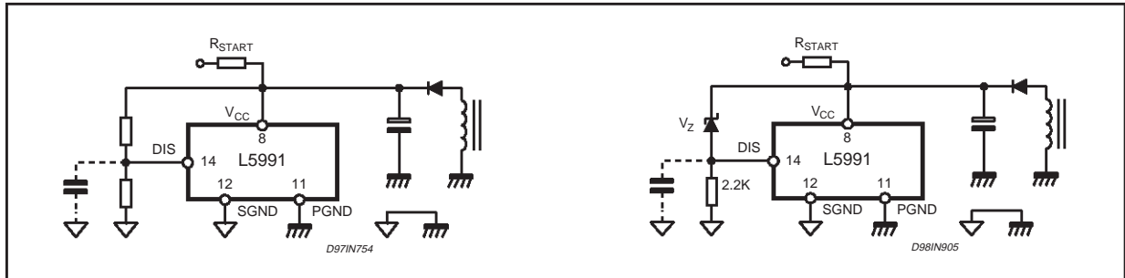
Figure 42 Protection against overvoltage/feedback disconnection (not latched)
