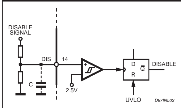
Figure 29. Disable (Latched).
