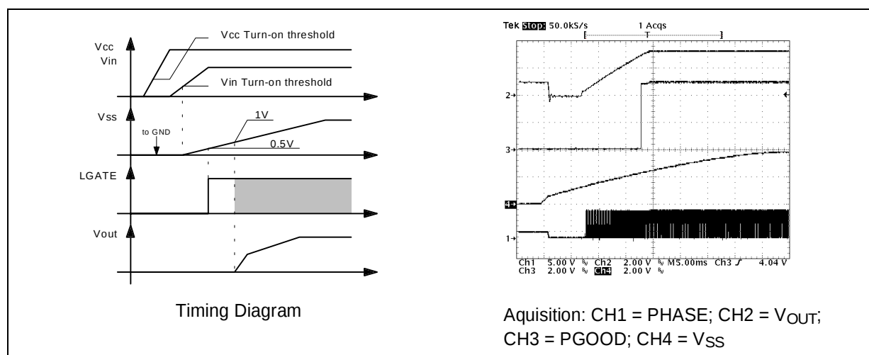
Figure 2. Soft Start
