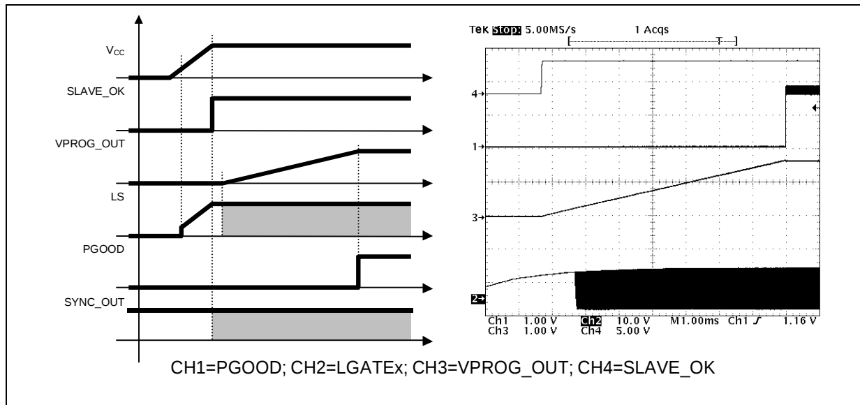
Figure 3. Soft Start
