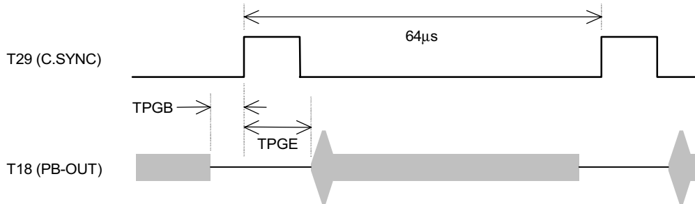
Fig.3 PB mode sync gate timing
