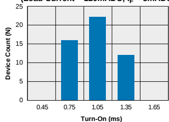
LBA110 - FormA Typical Turn-On Time (N=50 Ambient Temperature = 25°C) (Load Current = 120mADC; I_F = 5\text{mADC} )
