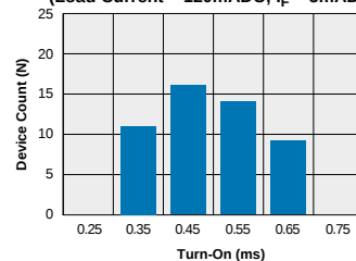
LBA110 - FormB Typical Turn-On Time (N=50 Ambient Temperature = 25°C) (Load Current = 120mADC; I_F = 5\text{mADC} )
