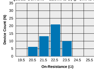
LBA110 - FormA Typical On-Resistance Distribution (N=50 Ambient Temperature = 25°C) (Load Current = 120mADC, I_F = 5\text{mADC} )
