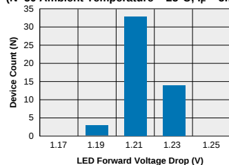
LBA110 Typical LED Forward Voltage Drop (N=50 Ambient Temperature = 25°C; I_F = 5\text{mADC} )
