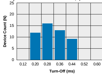
LBA110 - FormA Typical Turn-Off Time (N=50 Ambient Temperature = 25°C) (Load Current = 120mADC; I_F = 5\text{mADC} )
