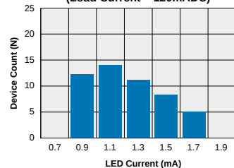
LBA110 - FormB Typical I_F for Switch Dropout (N=50 Ambient Temperature = 25°C) (Load Current = 120mADC)
