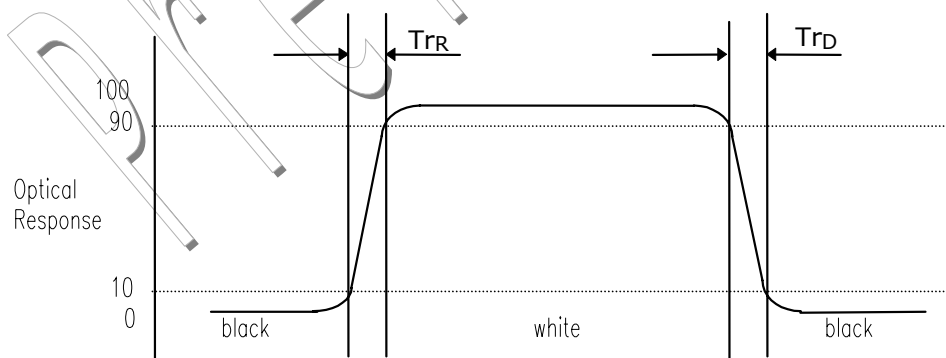
FIG. 3 Response Time
