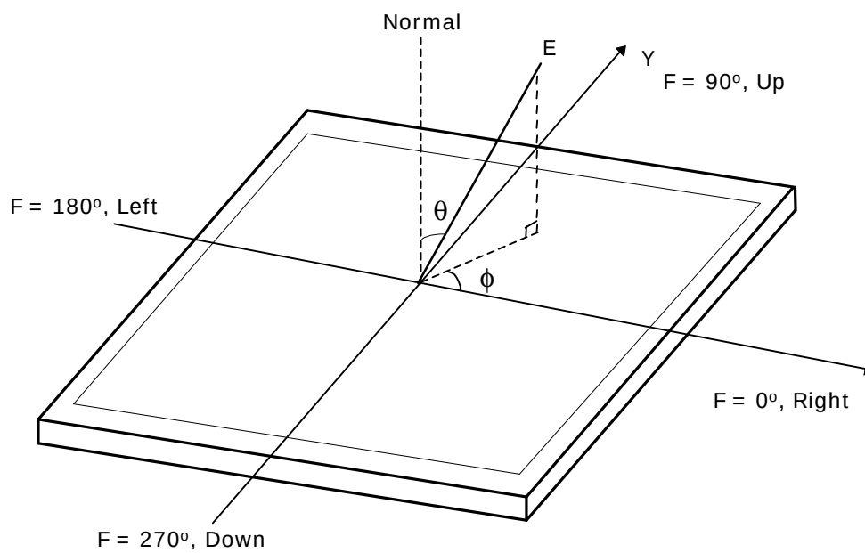
FIG. 4 Viewing angle
