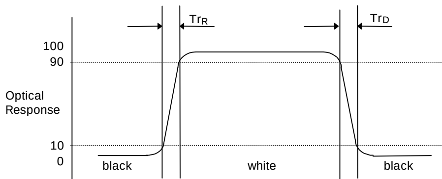
FIG. 3 Response Time
