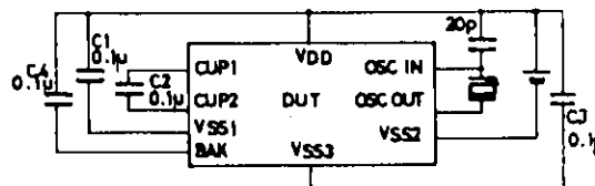
Fig. 11 Output voltage, current dissipation, oscillation hold voltage test circuit
