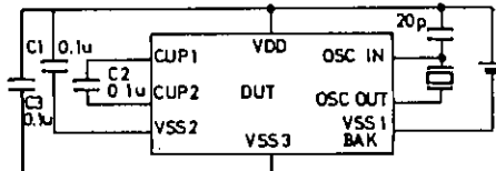
Fig. 7 Supply Current, Oscillation Hold Voltage Test Circuit
