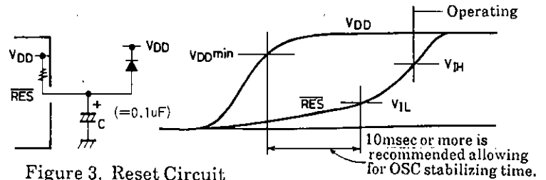
Figure 3. Reset Circuit
