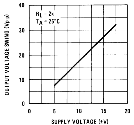
Voltage Swing
