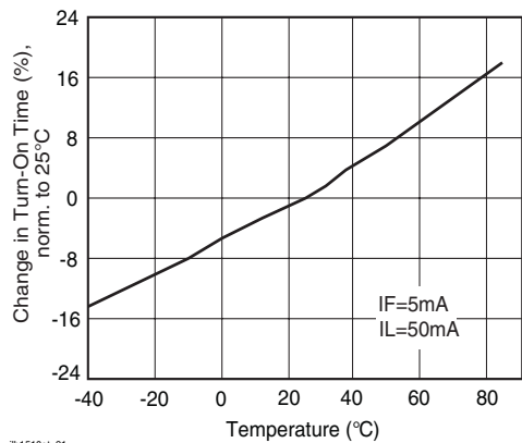
Figure 22. Turn-on Time vs. Temperature
