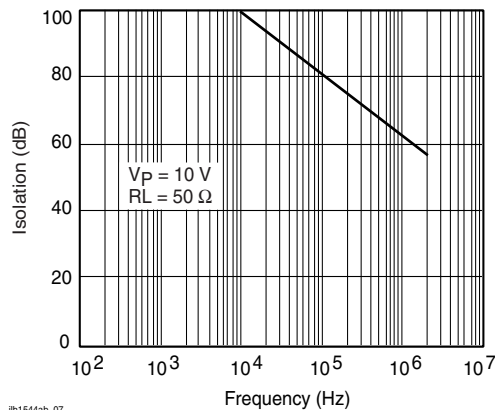
Figure 8. Output Isolation
