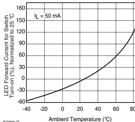
Figure 4. LED Current for Switch Turn-on vs. Temperature
