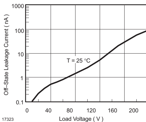
Figure 9. Leakage Current vs. Applied Voltage
