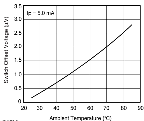
Figure 12. Switch Offset Voltage vs. Temperature
