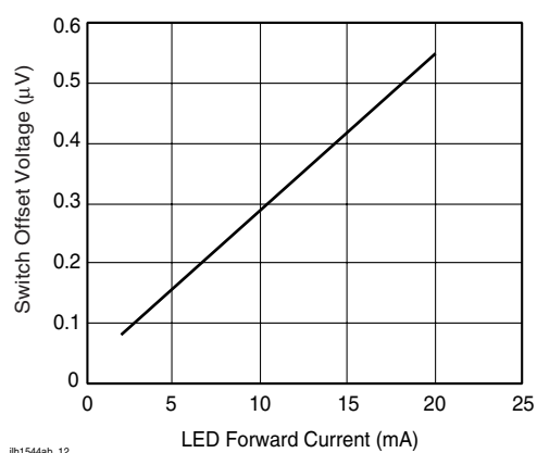
Figure 13. Switch Offset Voltage vs. LED Current
