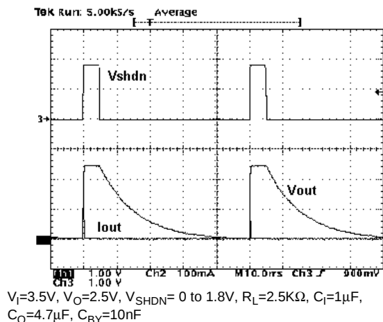
Figure 21 : Start-up Transient
