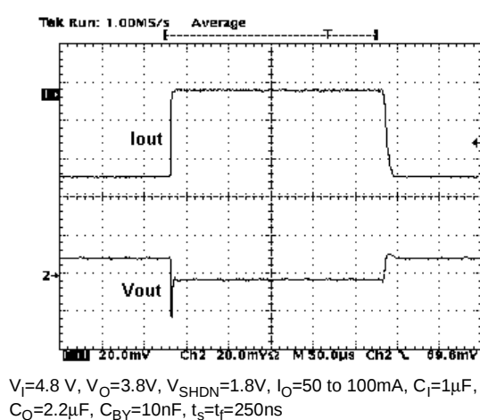
Figure 28 : Load Transient
