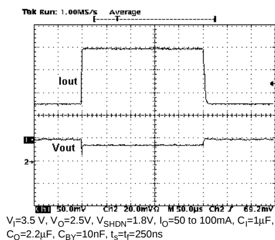
Figure 26 : Load Transient
