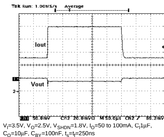
Figure 28 : Load Transient
