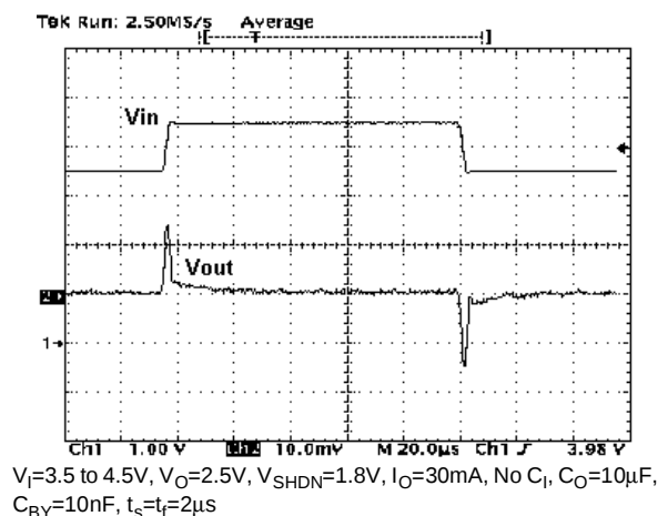
Figure 24 : Line Transient
