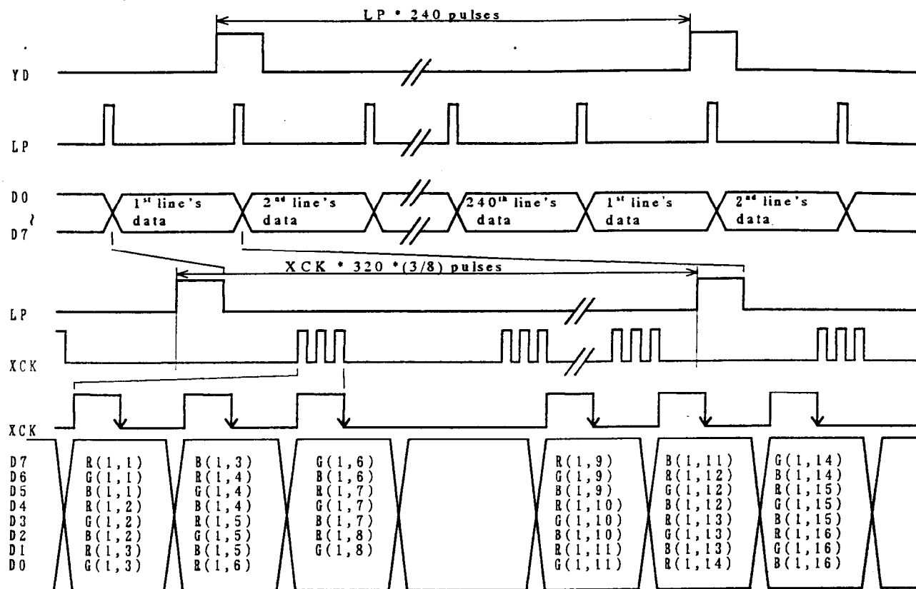
Fig.2 Interface timing
