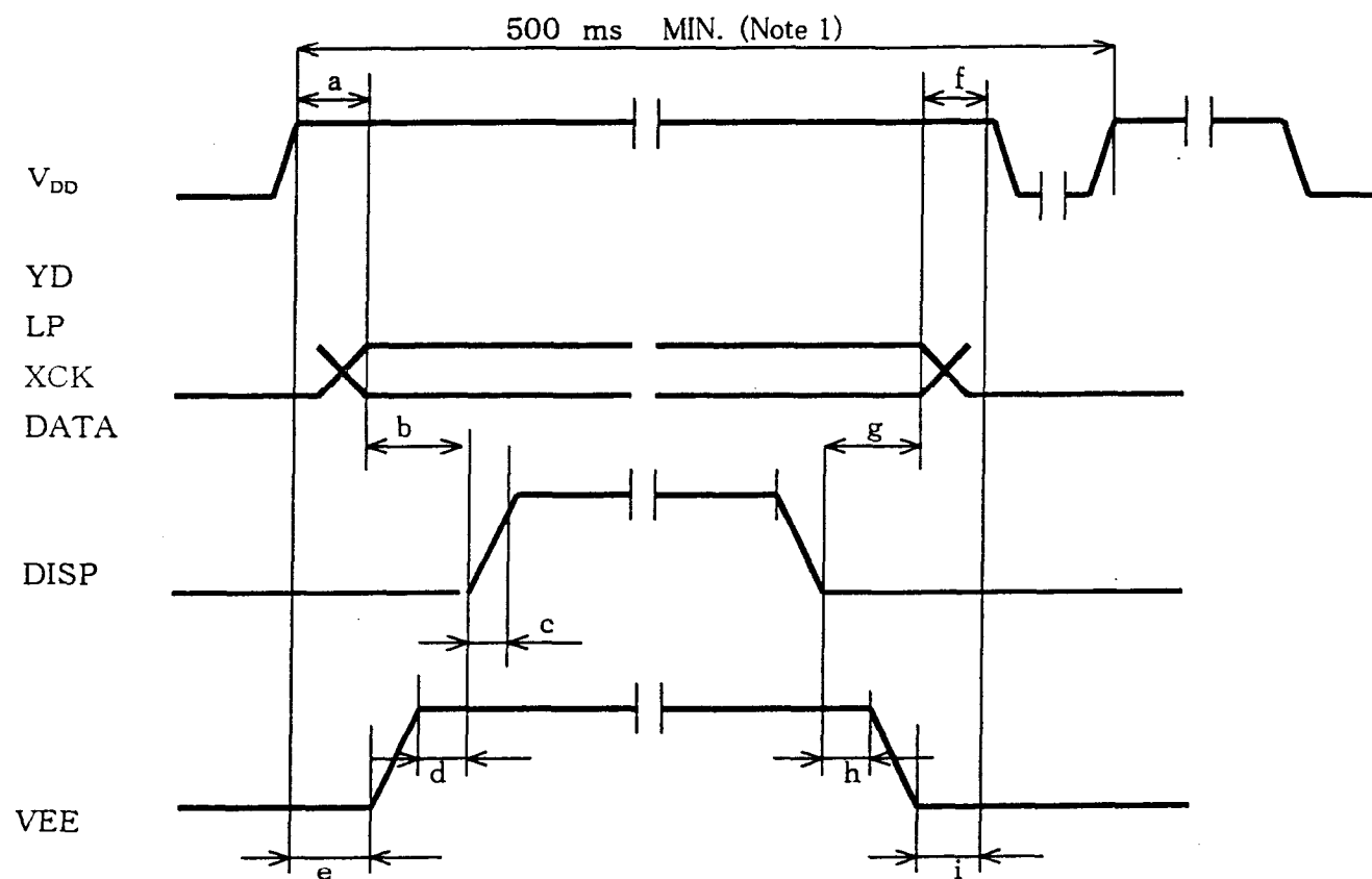
Fig.12 Sequence condition
