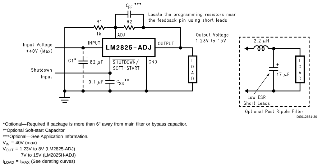
FIGURE 3. Standard Test Circuit (Adjustable Output Voltage Versions)
