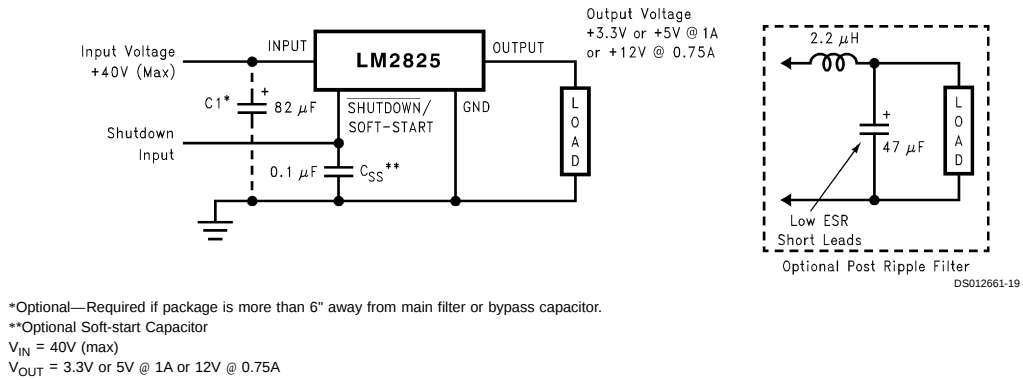
FIGURE 2. Standard Test Circuit (Fixed Output Voltage Versions)
