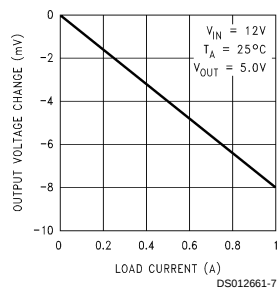
Load Regulation
