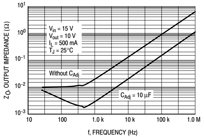
Figure 14. Output Impedance
