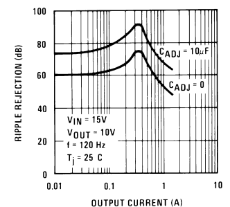
Ripple Rejection
