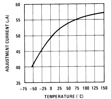
Adjustment Current
