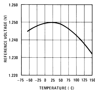
Temperature Stability
