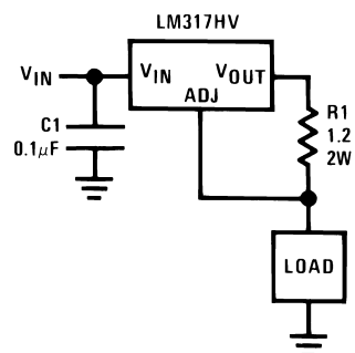
1A Current Regulator
