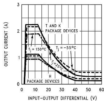
Current Limit
