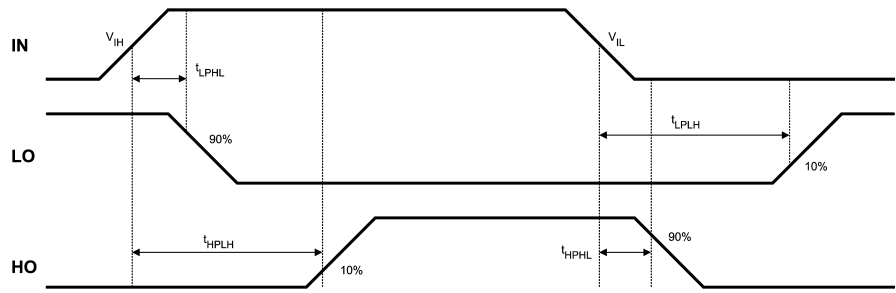
LM5105 Switching Time Definitions: t_{LPLH} , t_{LPHL} , t_{HPLH} , t_{HPLH}
