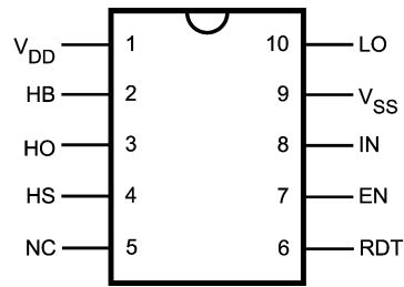
20137501 10-Lead LLP See NS Number SDC10A
