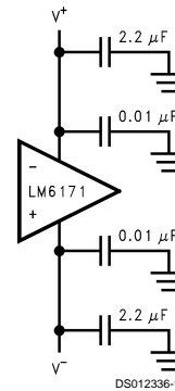
FIGURE 2. Power Supply Bypassing
