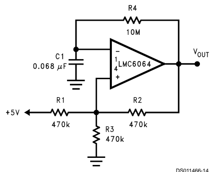
FIGURE 9. 1 Hz Square Wave Oscillator
