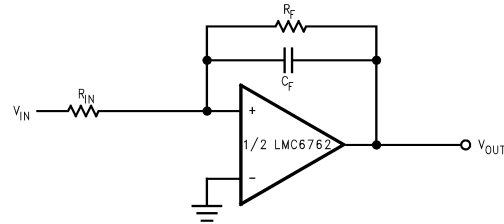
FIGURE 5. Canceling the Effect of Input Capacitance
