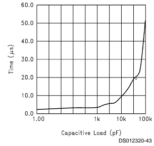
Response Time vs Capacitive Load
