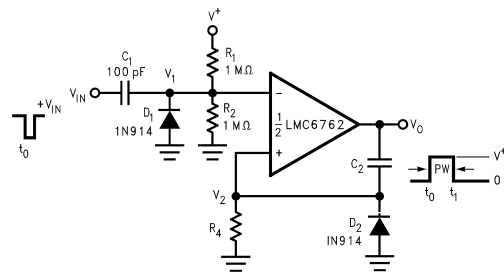
FIGURE 6. One-Shot Multivibrator
