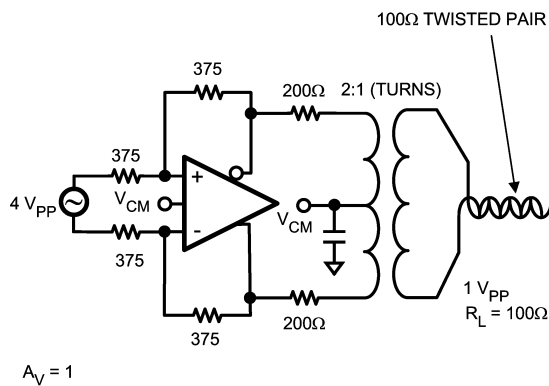
FIGURE 11. Transformer Out Low Impedance Load
