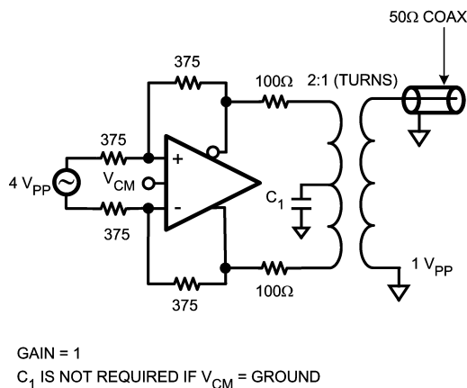
FIGURE 12. Driving 50Ω Test Equipment
