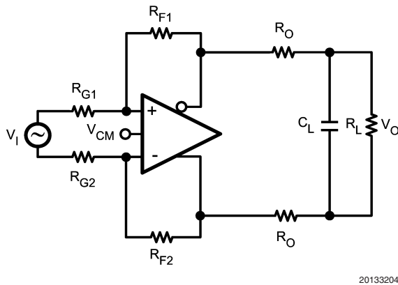
FIGURE 1. Typical Application
