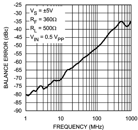
Balance Error
