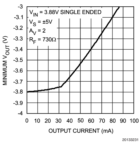
Minimum VOUT vs. IOUT
