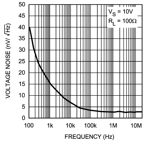
Voltage Noise
