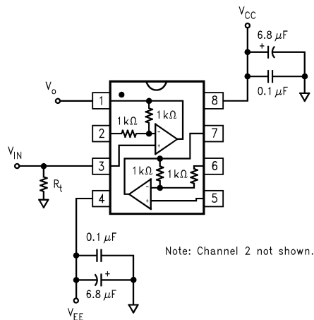
FIGURE 8. Dual Supply, A_V = +1V/V Configuration
