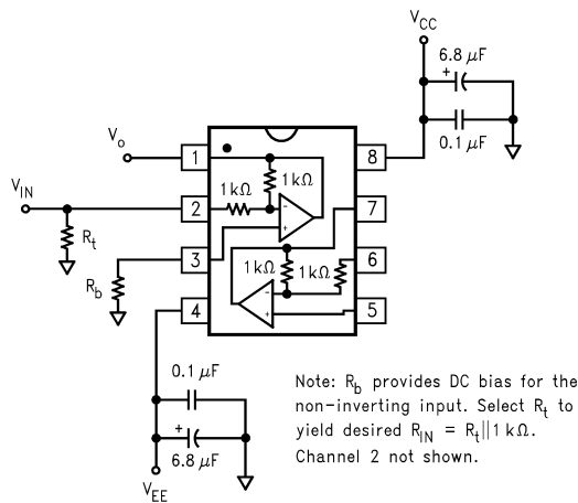
FIGURE 7. Dual Supply, A_V = -1V/V Configuration
