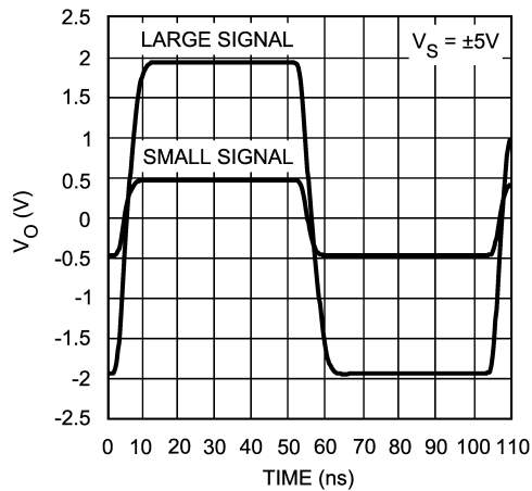
Pulse Response
