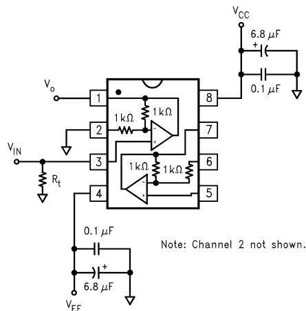
FIGURE 9. Dual Supply, A_V = +2V/V Configuration
