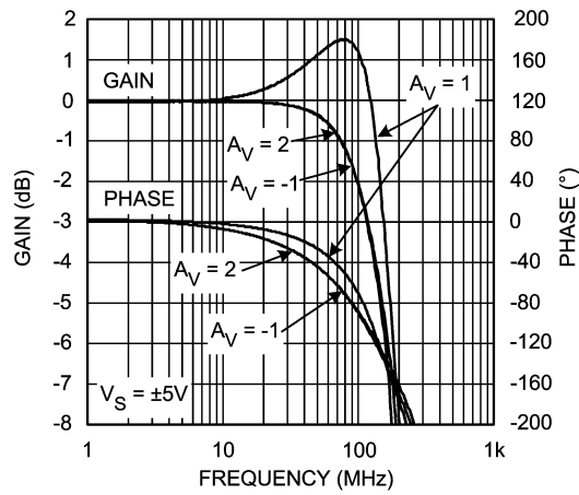
Frequency Response vs. Gain
