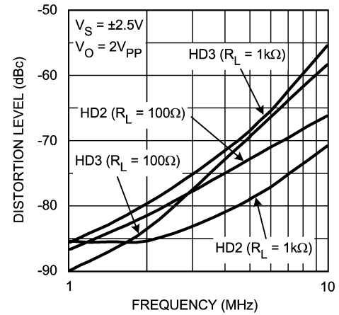
2nd & 3rd Harmonic Distortion vs. Frequency
