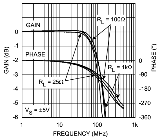
Frequency Response R_L
