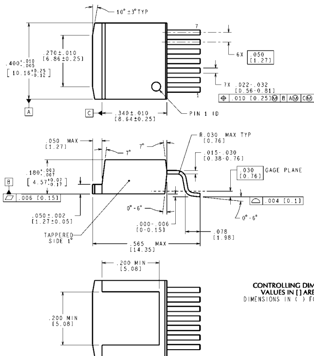
7-Pin TO-263 NS Package Number TS7B
