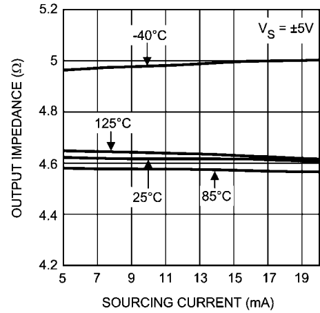
Output Impedance vs. Sourcing Current
