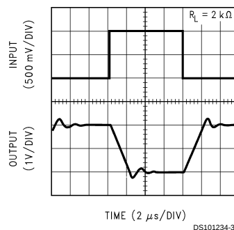
Inverting Large Signal Pulse Response LMV102
