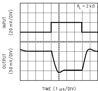
Inverting Small Signal Pulse Response LMV105
