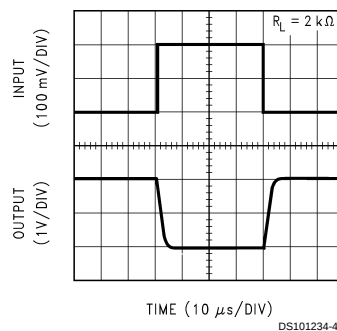
Inverting Large Signal Pulse Response LMV110
