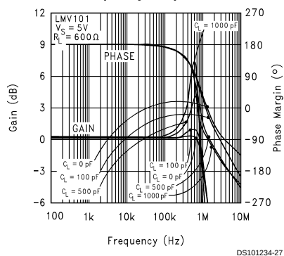
LMV101 Close Loop Frequency Response
