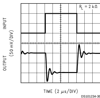
Inverting Small Signal Pulse Response LMV101
