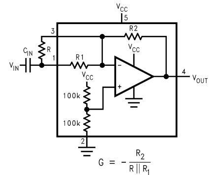
FIGURE 8. Increased Gain
