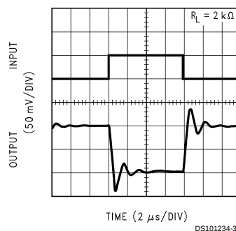
Inverting Small Signal Pulse Response LMV102
