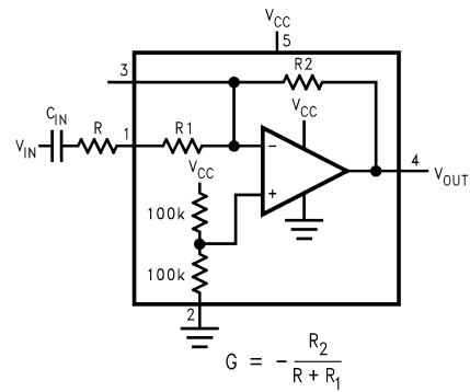
FIGURE 7. Decreased Gain
