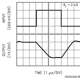
Inverting Large Signal Pulse Response LMV105
