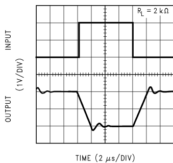
Inverting Large Signal Pulse Response LMV101
