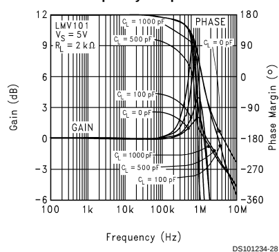
LMV101 Close Loop Frequency Response
