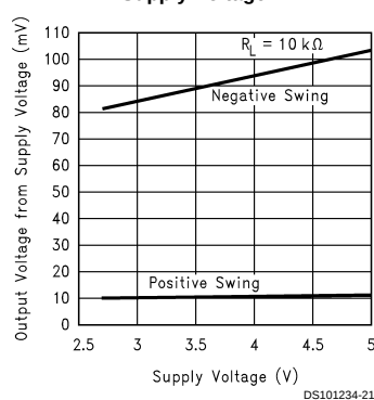
Output Voltage Swing vs. Supply Voltage
