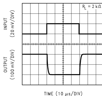
Inverting Small Signal Pulse Response LMV110
