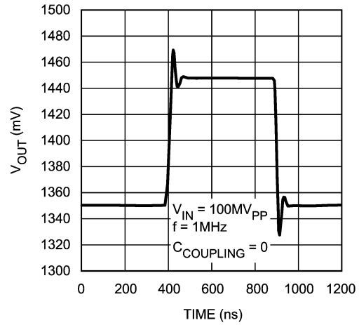
Small Signal Pulse Response
