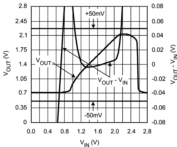
FIGURE 3. V_{OUT} - V_{IN}
