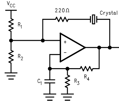
FIGURE 5. Crystal Oscillator
