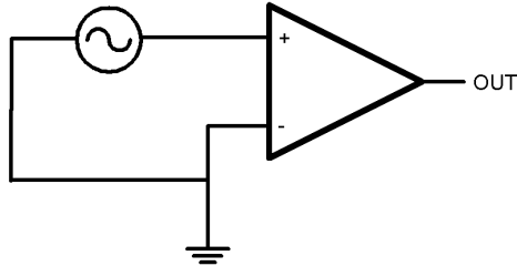
FIGURE 3. Zero-Crossing Detector
