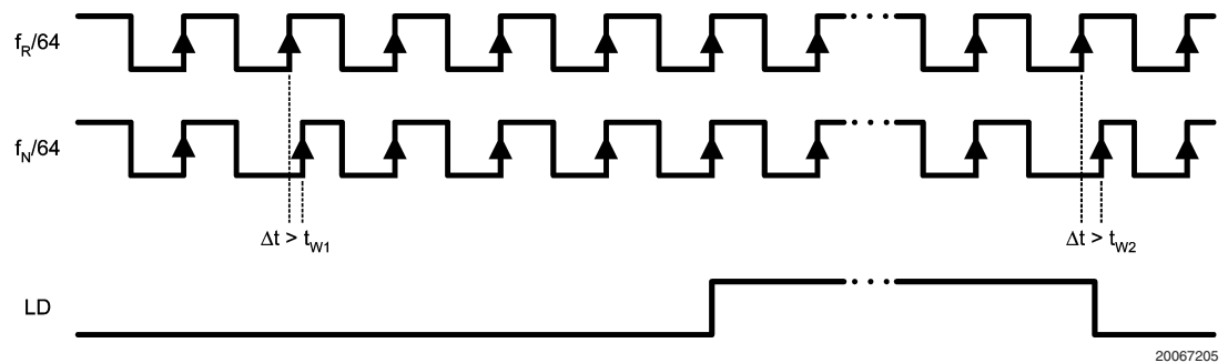
FIGURE 1. Lock Detect Timing Diagram Waveform
