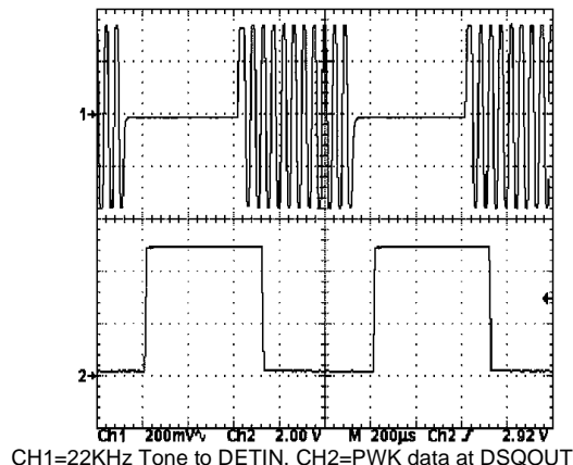
Figure 8: DETIN/DSQOUT Waveform
