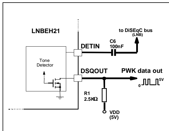
Figure 7: DETIN/DSQOUT Circuit
