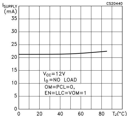
Figure 15: Supply Current vs Temperature
