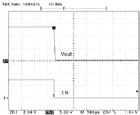
Disable Time
