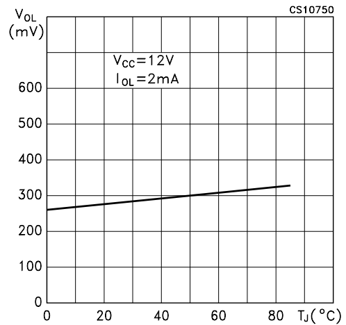
Figure 25 : DSQOUT Pin Logic Low vs Temperature
