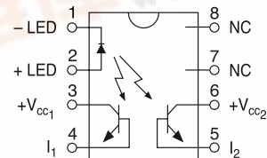
LOC111 Pinout
