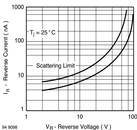
Fig. 3 Reverse Current vs. Reverse Voltage
