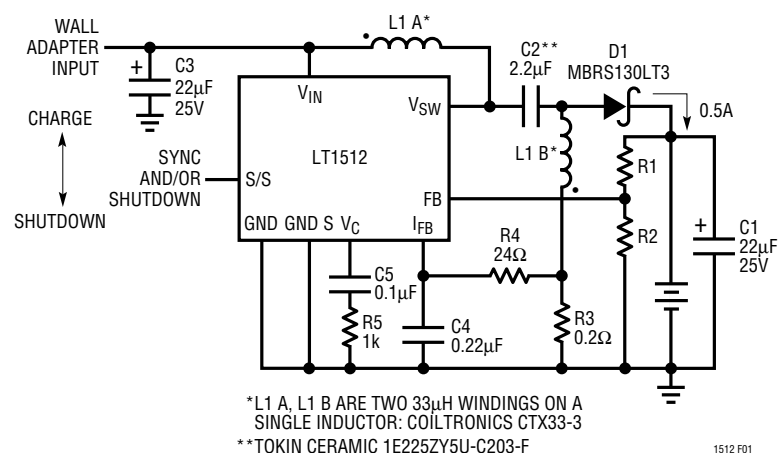
Figure 1. SEPIC Charger with 0.5A Output Current
