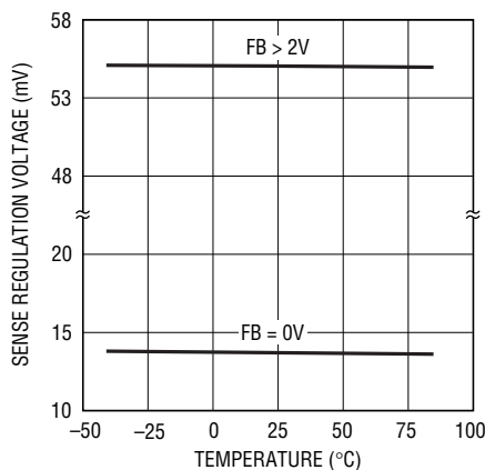
SENSE Regulation Voltage vs Temperature
