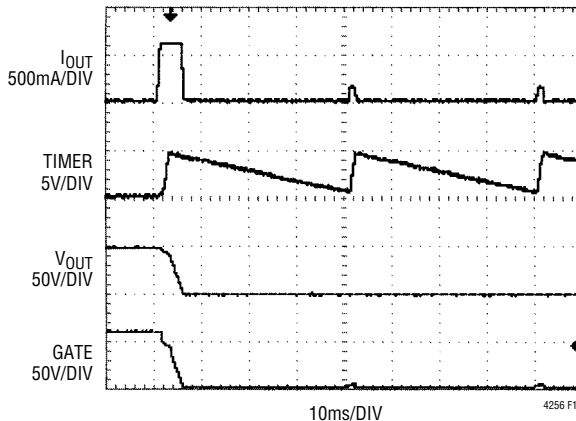
Figure 11. RETRY Waveforms
