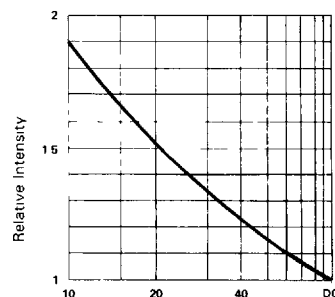
Duty Cycle % (AVERAGE I_F = 10\text{ mA PER SEG} ) Fig 6 LUMINOUS INTENSITY Vs DUTY CYCLE %
