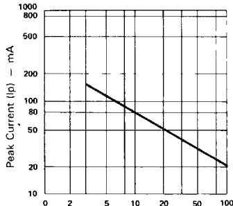
Duty Cycle % (REFRESH RATE F = 1\text{ KHz} ) Fig 5 MAX PEAK CURRENT Vs DUTY CYCLE %
