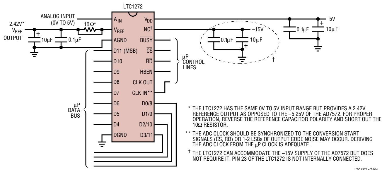
Figure 22. Plugging the LTC1272 into an AD7572 Socket Case 1: Clock Synchronous with \overline{\text{CS}} and \overline{\text{RD}}
