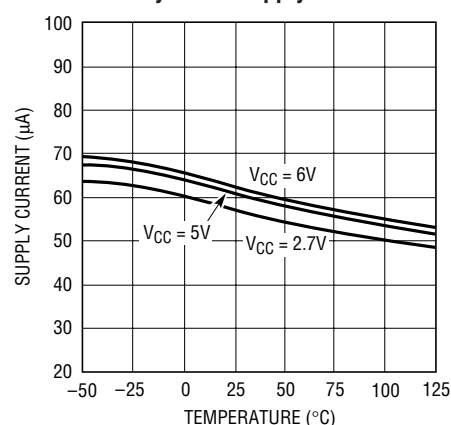
Standby Mode Supply Current
