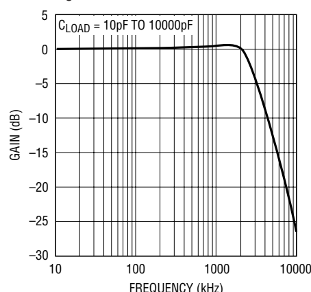
V_{OCM} Gain vs Frequency, V_S = \pm 2.5V
