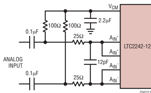
Figure 5. Capacitively-Coupled Drive
