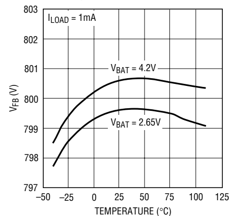
FB Pin Regulated Voltage vs Temperature
