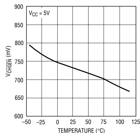
CHGEN Pin Threshold Voltage (On-to-Off) vs Temperature
