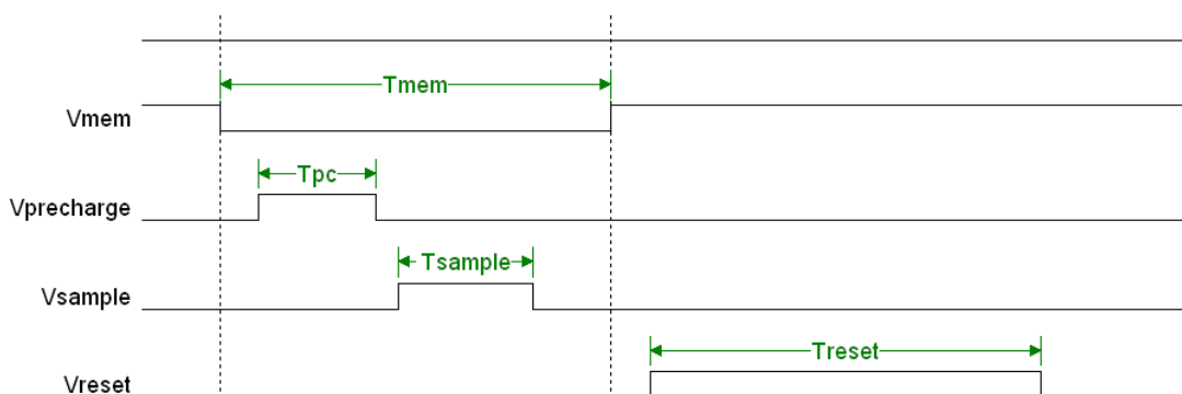
Figure 12: Internal timing of the pixel.
