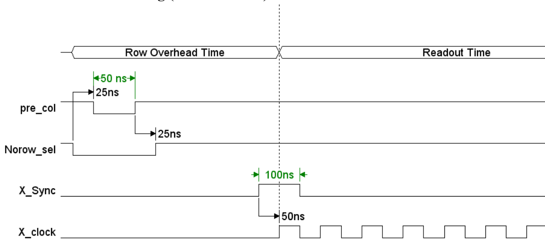
Figure 18: Only pre_col and Norowsel control signals are required. SH_col is made active low.
