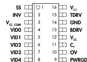
D PACKAGE — 16-Pin LX1663/1663A (Top View)
