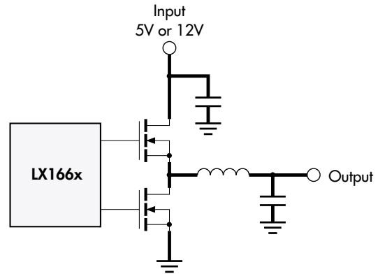
FIGURE 13 — Power Traces
