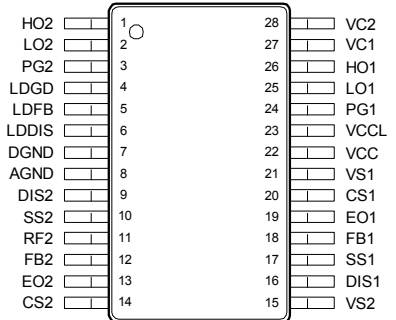
PW PACKAGE (Top View)
