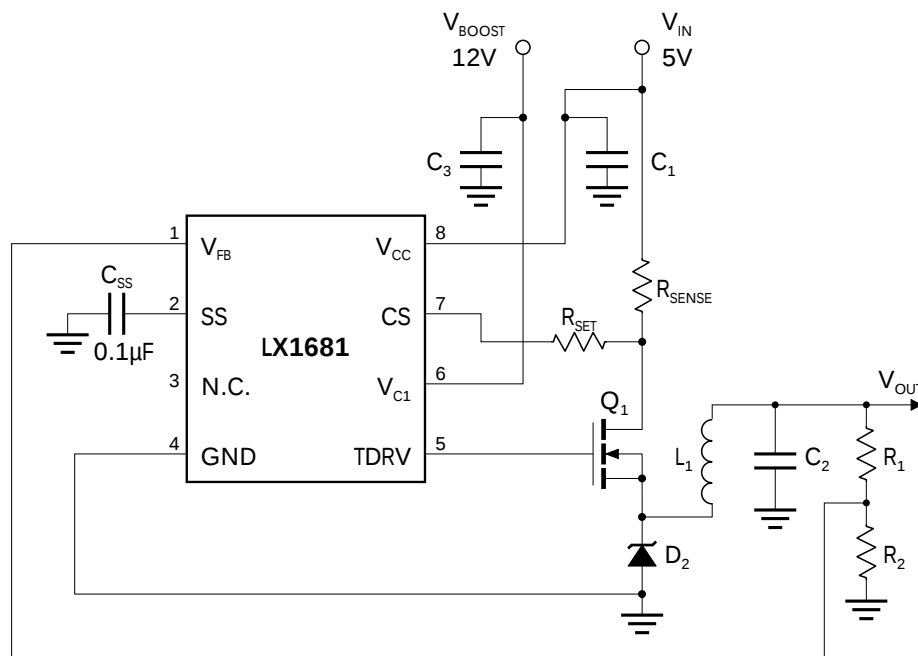
FIGURE 3 — Current Sensing Using Sense Resistor
