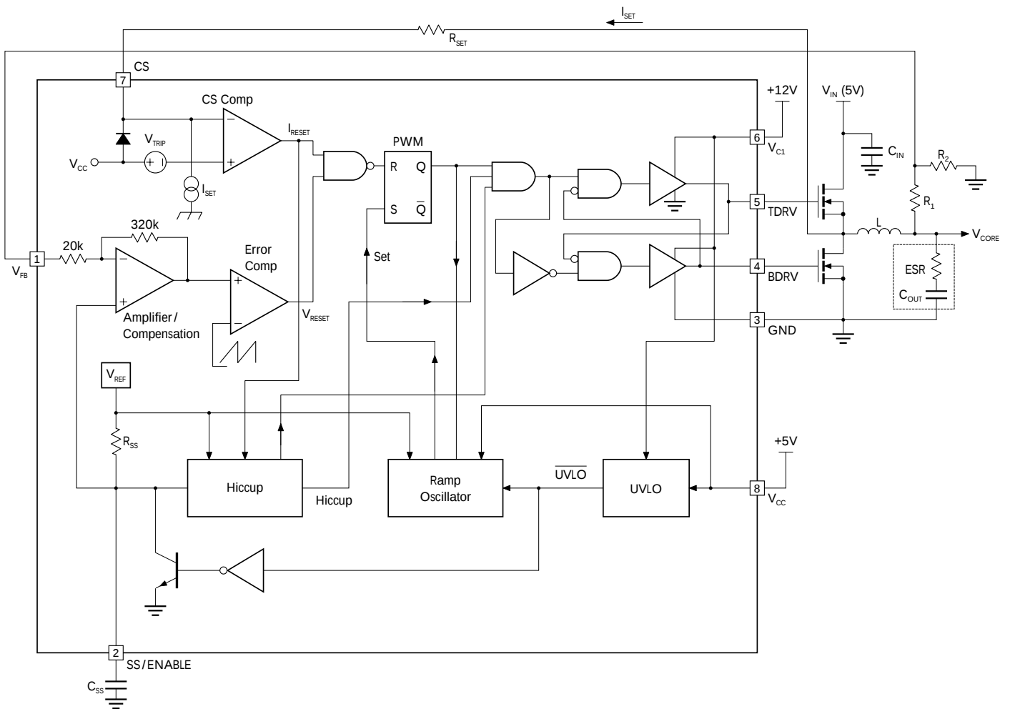
FIGURE 1 — Block Diagram
