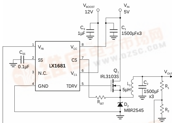
LX1681 Non-Synchronous Controller
