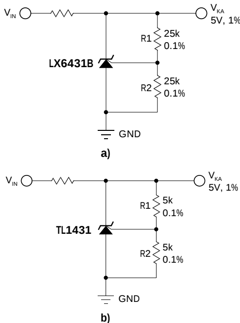
FIGURE 7 — Comparison of reference resistor values between an LX6431B and an TL1431, resistors used with the LX6431B are 5 times higher in value.
