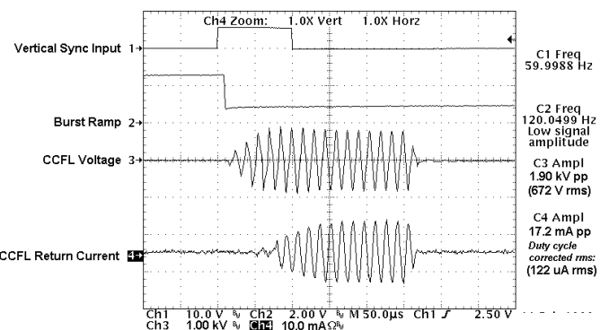
Figure 3 – 2% Burst Duty Cycle (Expanded Time Base)
